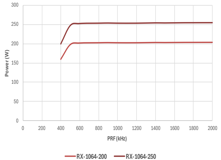
Power Vs. PRF
