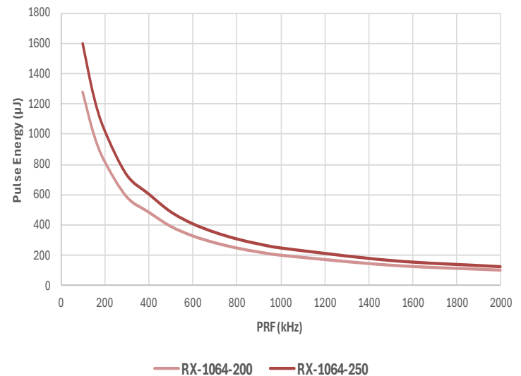
Pulse Energy Vs. PRF
